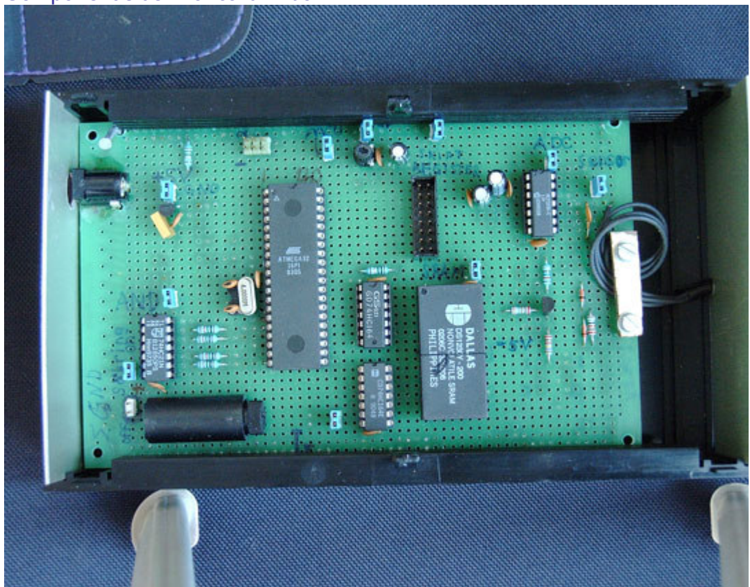
Component side final card in box
