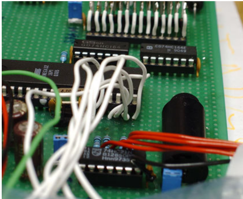
Component side final card in box
